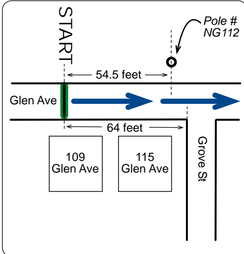
START DETAIL
